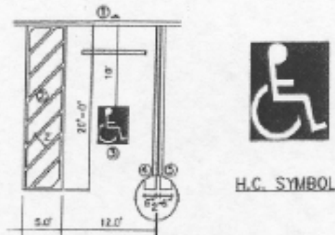
HANDICAP PARKING STRIPING AND PAVEMENT MARKING N.T.S.
