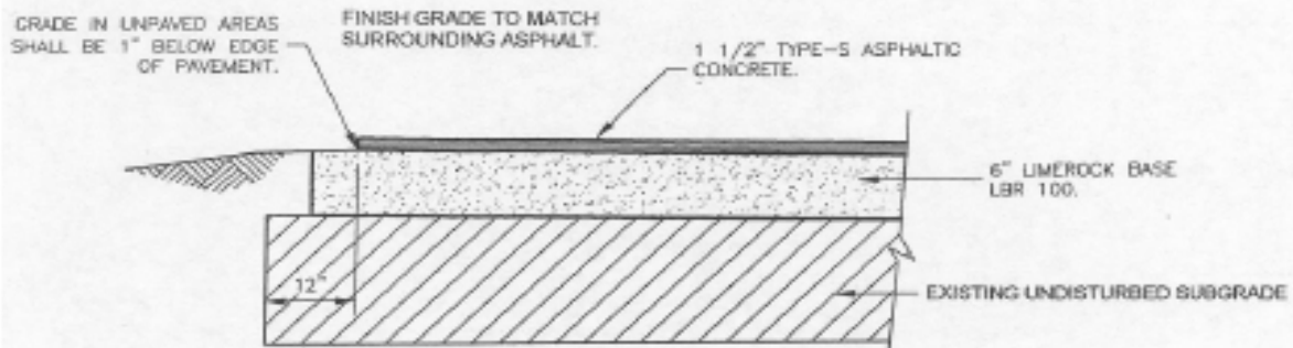
PAVEMENT PATCH & PARKING AREA TYPICAL SECTION N.T.S.
